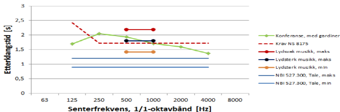
Figure 6: Reverberationtime conference setup with chairs
