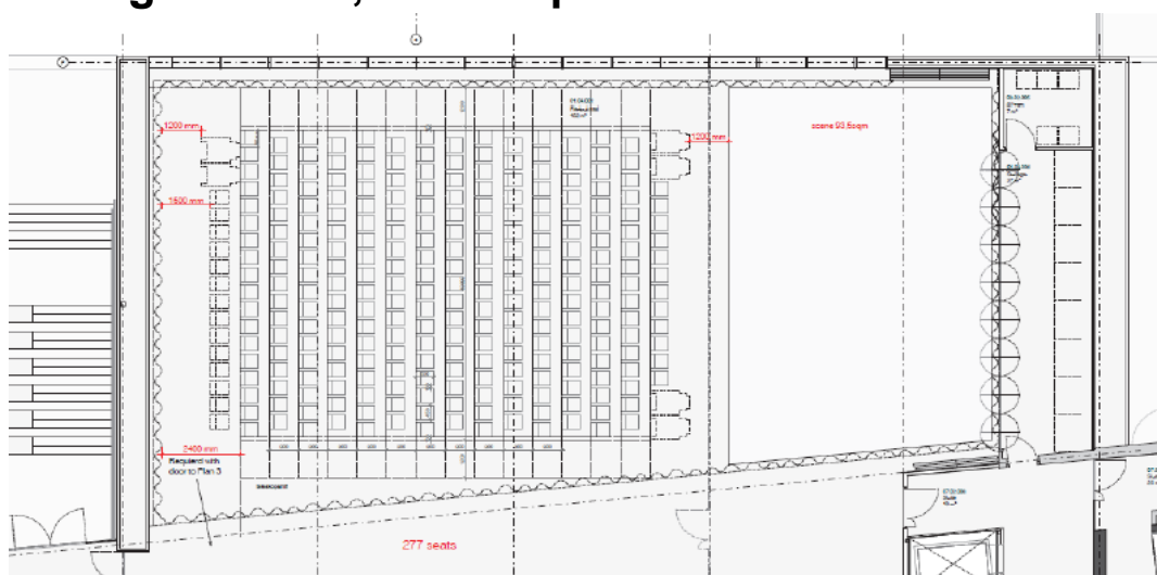
Figure 11: Setup telescopic bleachers
